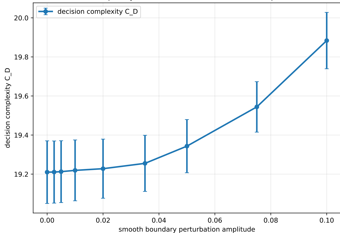
Structural complexity remains controlled under smooth perturbations
