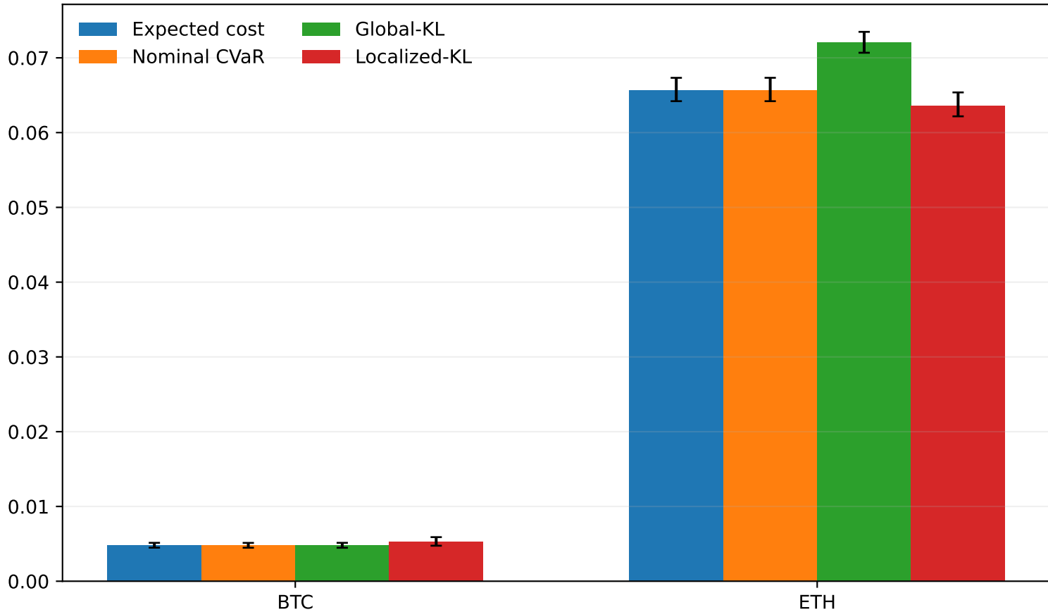
CVaR95 implementation shortfall (bps)
