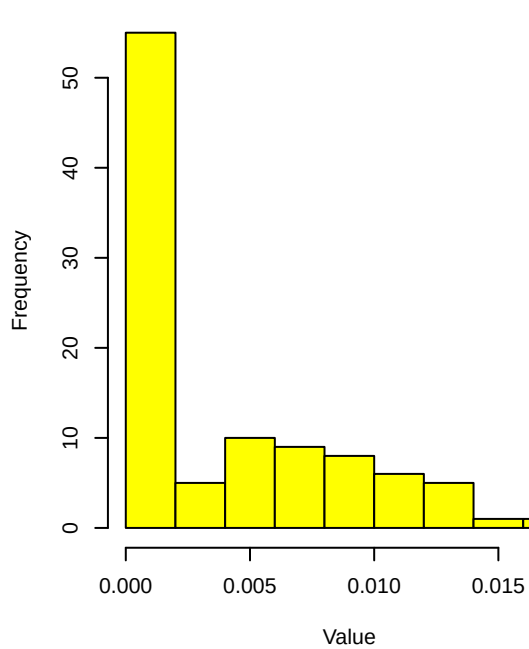
rmsea.scaled
