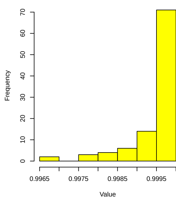
cfi.scaled
