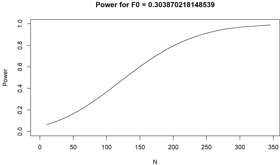
Figure 7: Power as a function of sample size for the population model (popModel)
