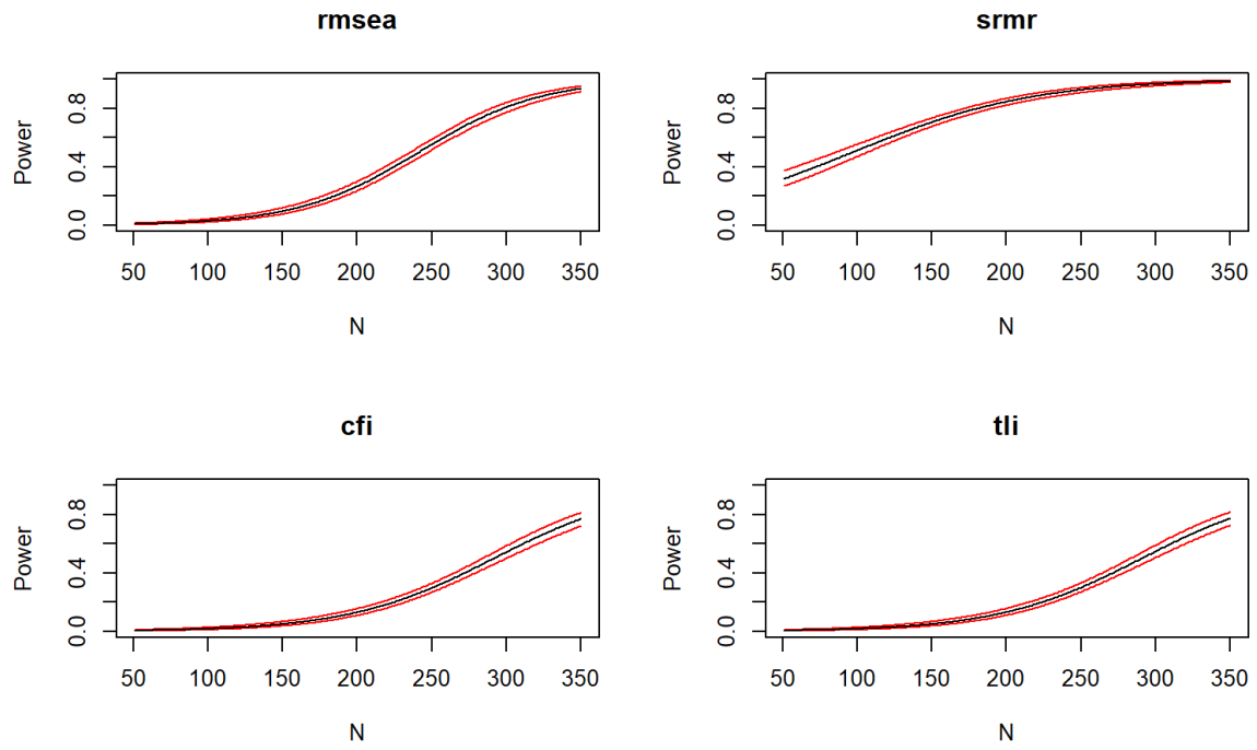
Figure 17: Power curves for fit indices under missing data conditions.
