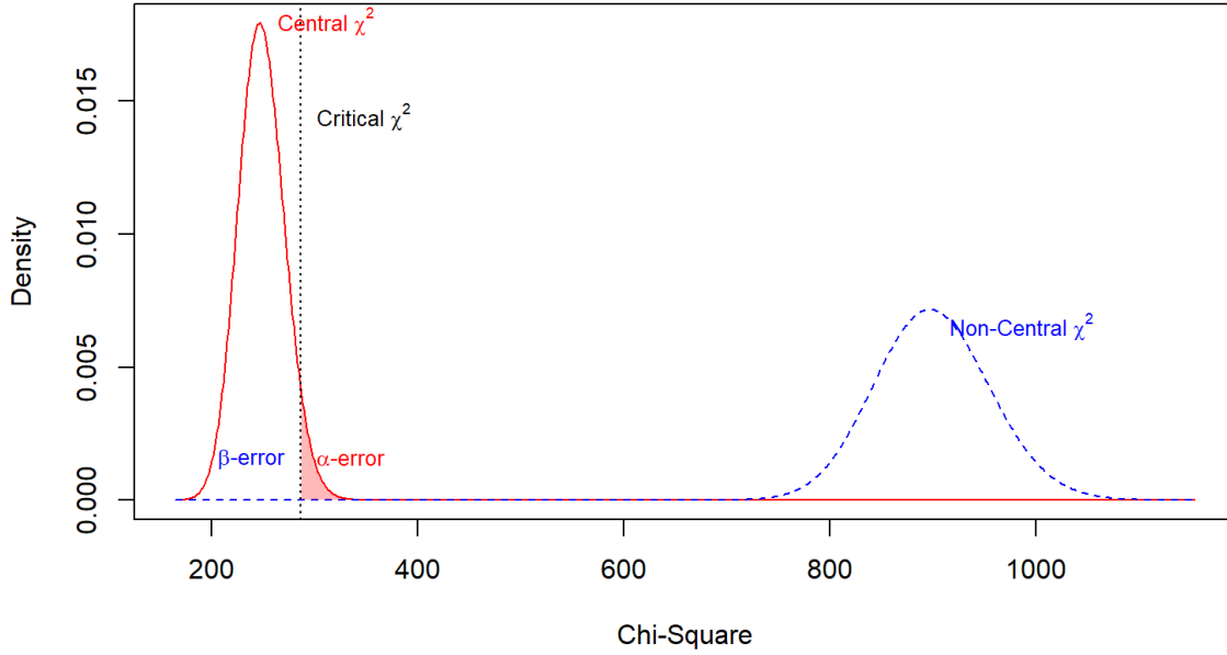
Figure 24: Post hoc power analysis for RMSEA = 0.05.
