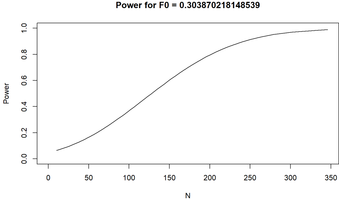
Figure 9: Power as a function of sample size for the population model (popModel)
