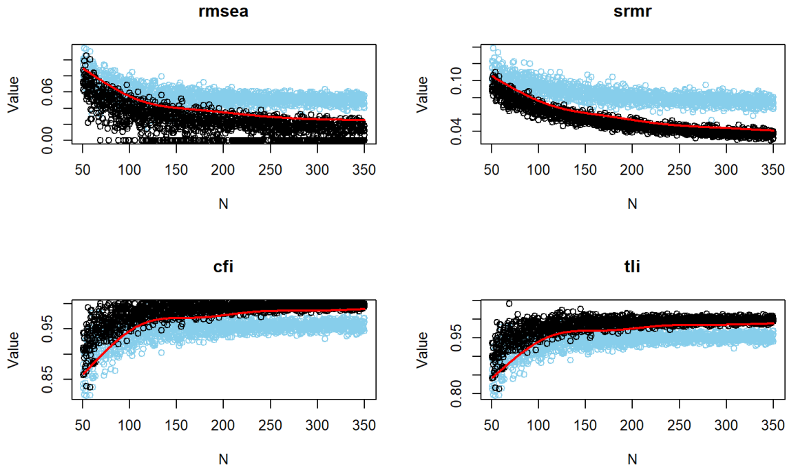
Figure 20: Power curves for fit indices under non-normal conditions without logistic smoothing.
