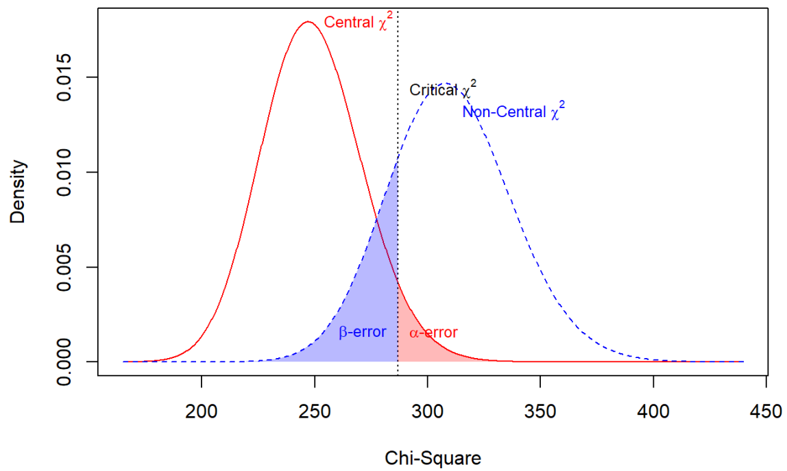
Figure 7: A priori power analysis Model-based approach (popModel)
