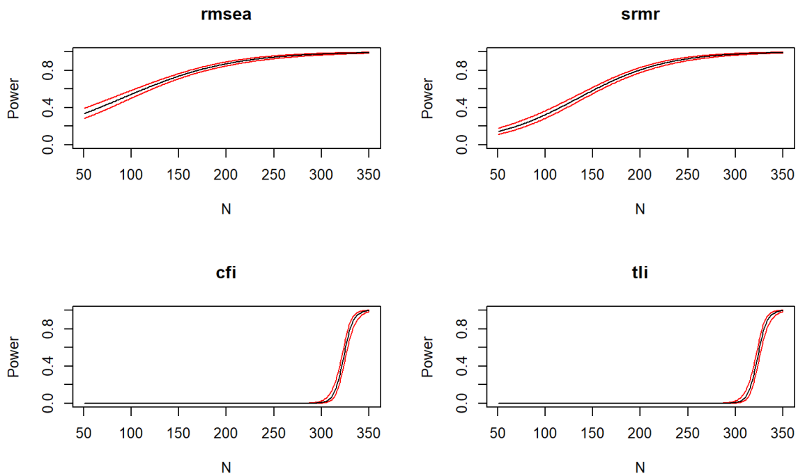
Figure 13: Power curves for fit indices using the naive population model.
