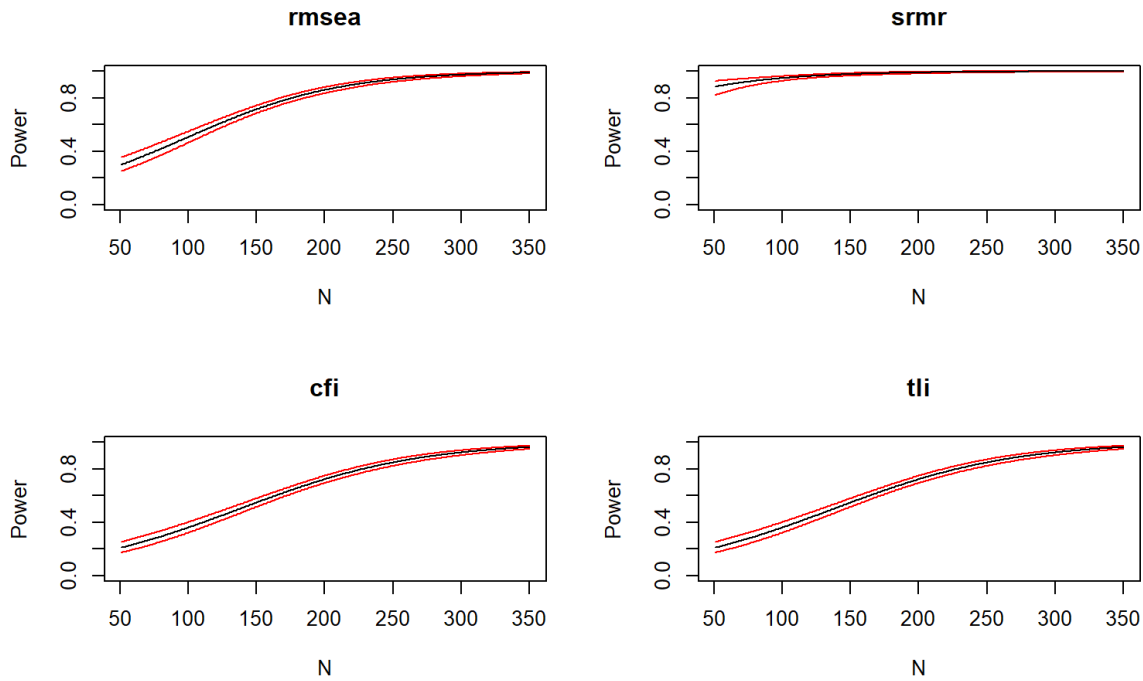
Figure 19: Power curves for fit indices under non-normal conditions.
