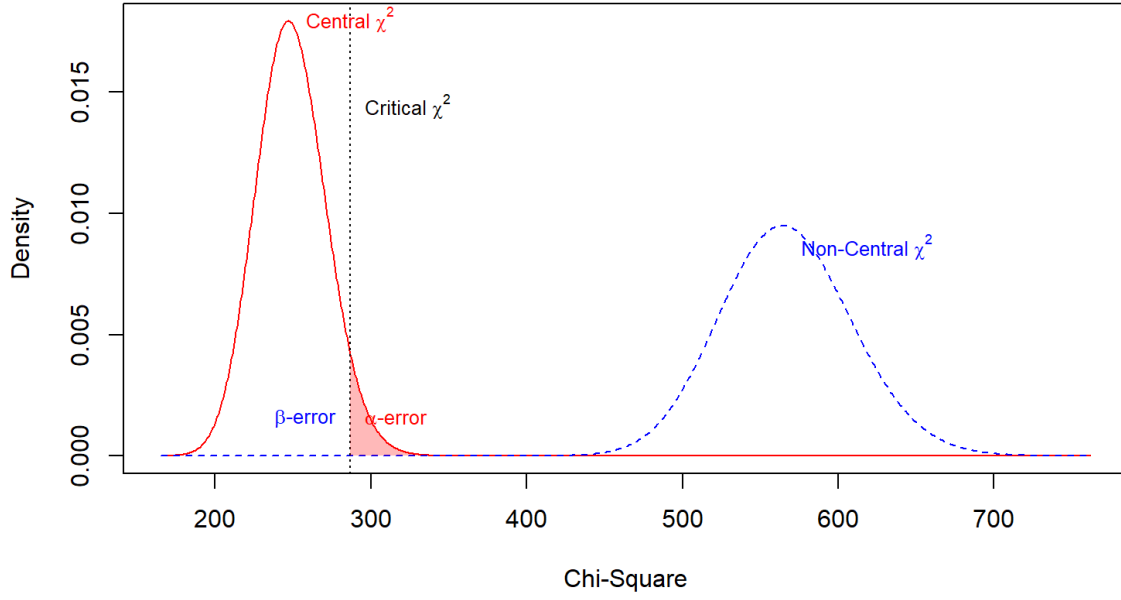
Figure 25: Post hoc power analysis for the real model.
