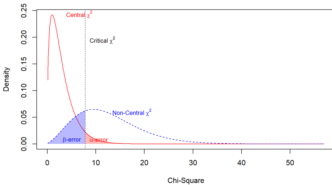
Figure 26: Post hoc power analysis for the misspecified model.
