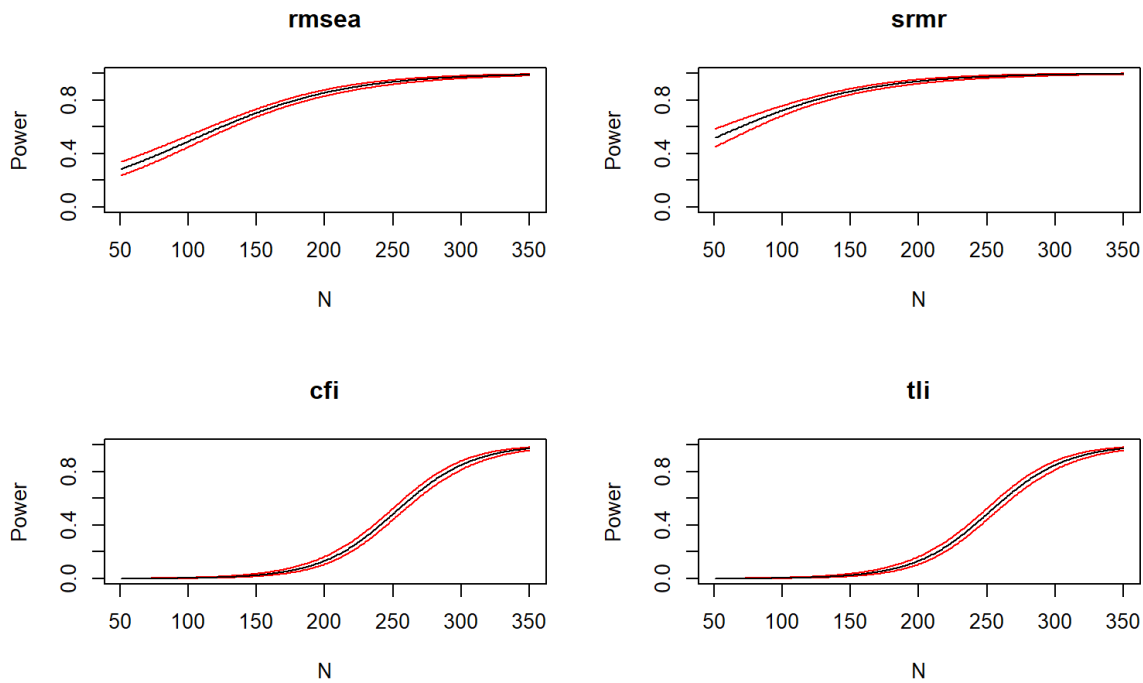
Figure 15: Power curves for fit indices using the optimal population model.
