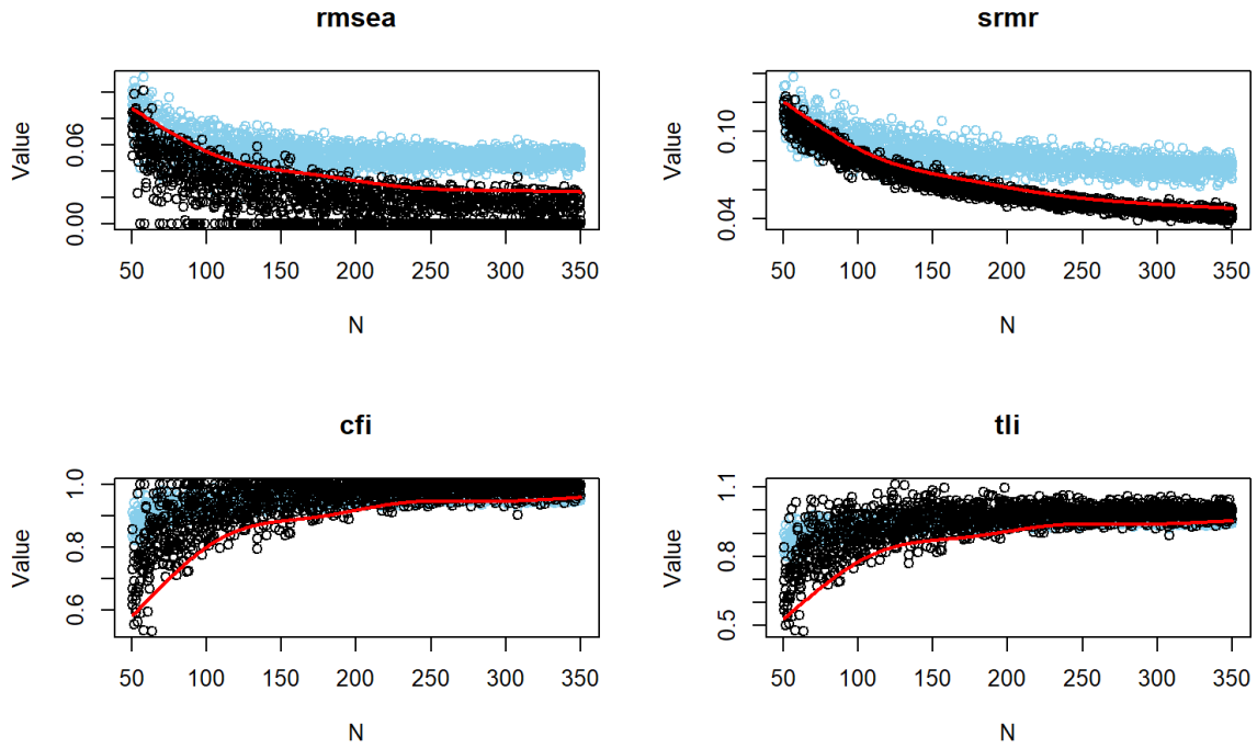
Figure 14: Power curves for fit indices using the naive population model without logistic smoothing.
