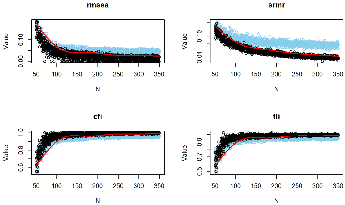
Figure 18: Power curves for fit indices under missing data conditions without logistic smoothing.
