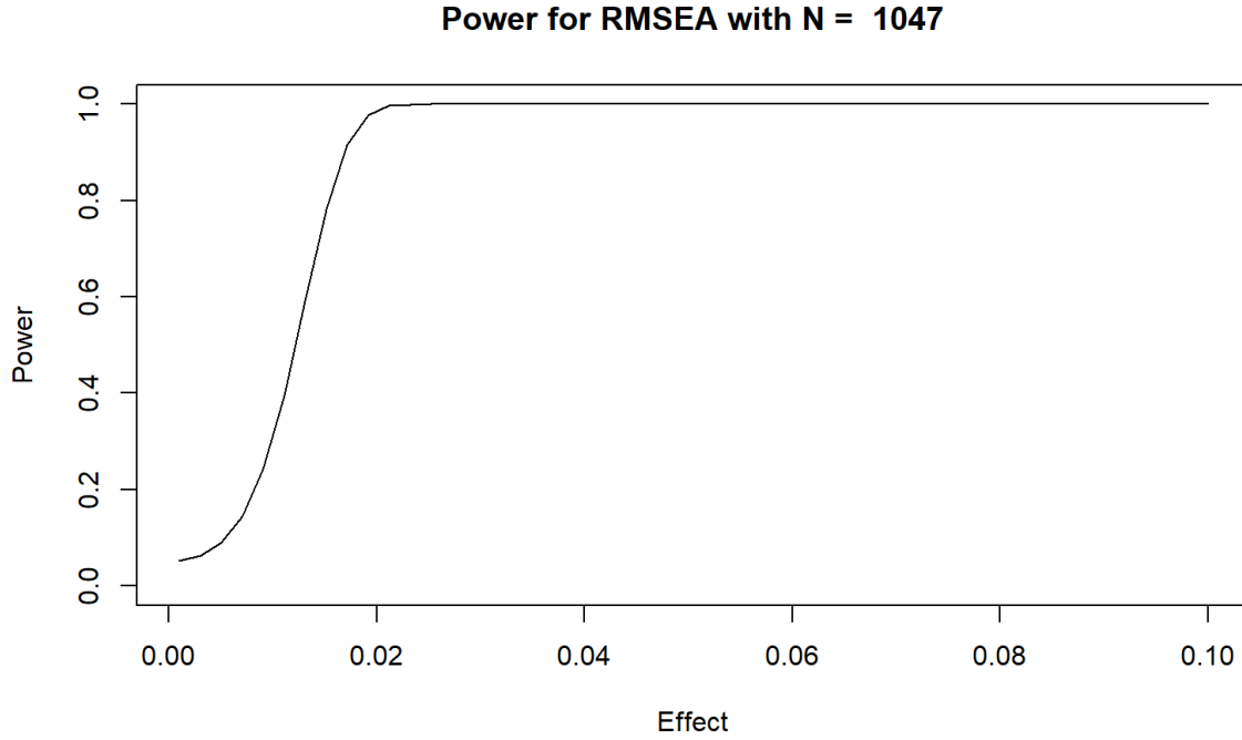
Figure 2: Power as a function of RMSEA magnitude with N = 1047
