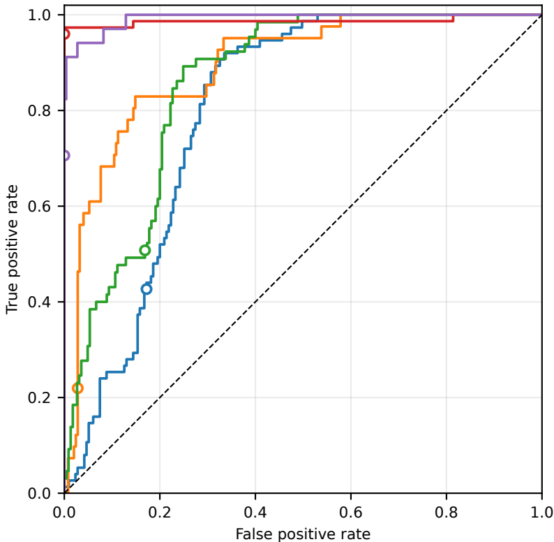
Per-family one-vs-rest ROC (known test set, seed 42)
