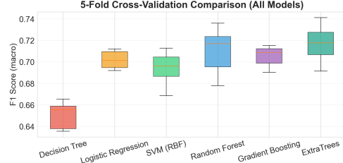
Figure 11: 5-fold CV comparison across model classes.
