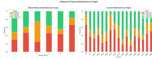
Figure 2: Categorical distributions stacked by target.
