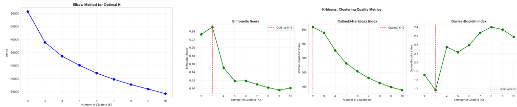
Figure 6: Left: Elbow method for K selection. Right: Silhouette, CH, and DB evaluation metrics vs. K.
