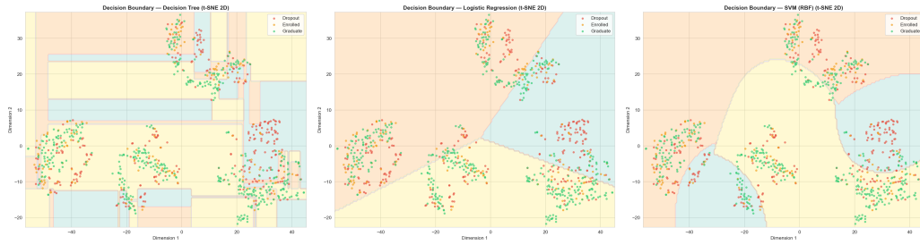
Figure 12: Approximate decision boundaries in t-SNE 2D space: DT (left), LR (center), SVM-RBF (right).
