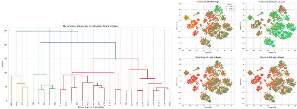
Figure 8: Left: Hierarchical clustering dendrogram (Ward linkage). Right: Comparison of clusters generated by Ward, Complete, Average, and Single linkages.
