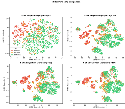
Figure 4: t-SNE 2D projections at perplexity = 5, 30, 50, 100.
