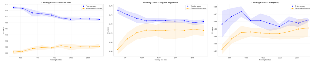
Figure 15: Learning curves: DT (left), LR (center), SVM (right).
