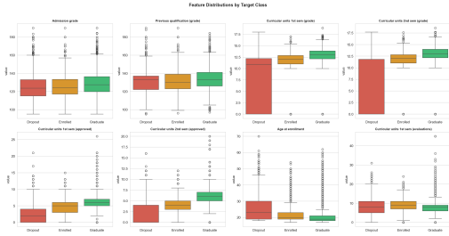
Figure 1: Feature distributions by target class.
