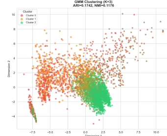
Figure 8: GMM (K=3)
