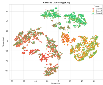
Figure 6: K-Means (K=3)
