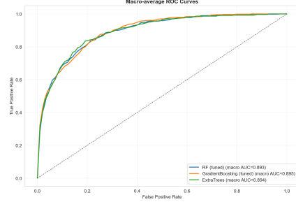
Figure 13: ROC curves for tuned RF, tuned GB, and ExtraTrees.
