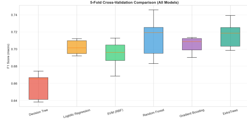
Figure 14: 5-fold CV comparison across model classes.
