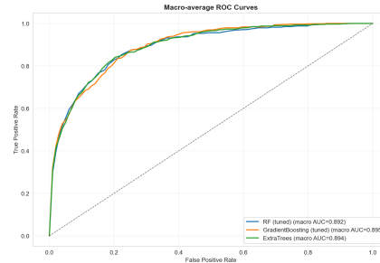
Figure 13: ROC curves for tuned RF, tuned GB, and ExtraTrees.
