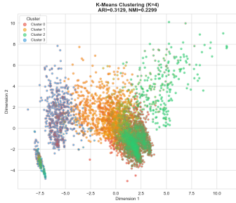
Figure 6: K-Means (K=4)
