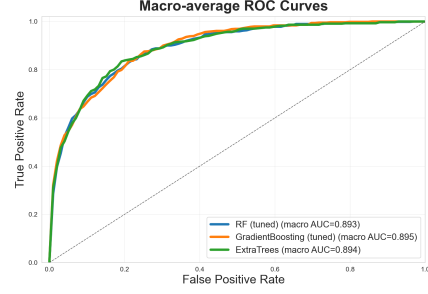
Figure 12: ROC curves for tuned RF, tuned GB, and ExtraTrees.
