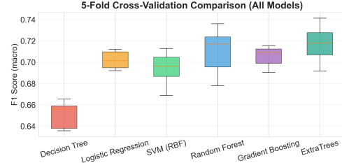
Figure 13: 5-fold CV comparison across model classes.
