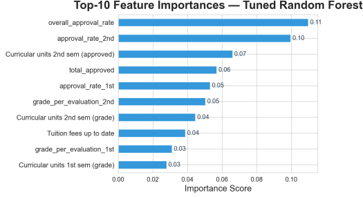
Figure 14: Top-10 feature importances from the tuned Random Forest.
