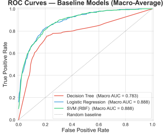
Figure 10: Macro-average ROC curves for all baseline models.
