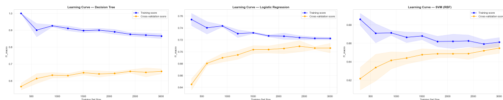
Figure 17: Learning curves: DT (left), LR (center), SVM (right).
