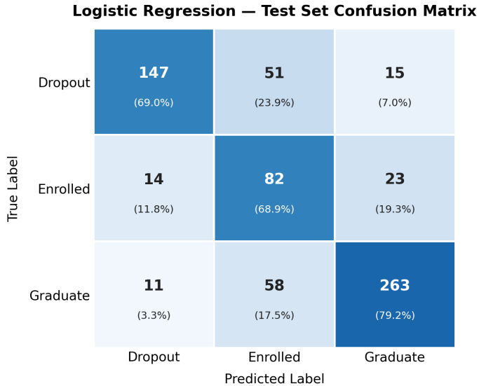
Figure 10: Logistic Regression confusion matrix on the test set. Enrolled students are most frequently misclassified (31.1% total error), confirming the class overlap discussed in Section 2.2–2.3.
