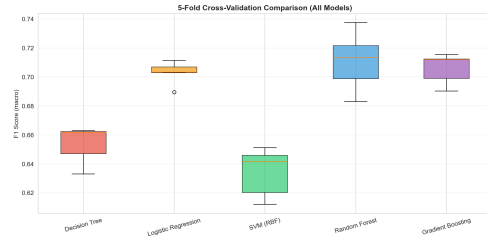
Figure 14: 5-fold CV comparison across all models.
