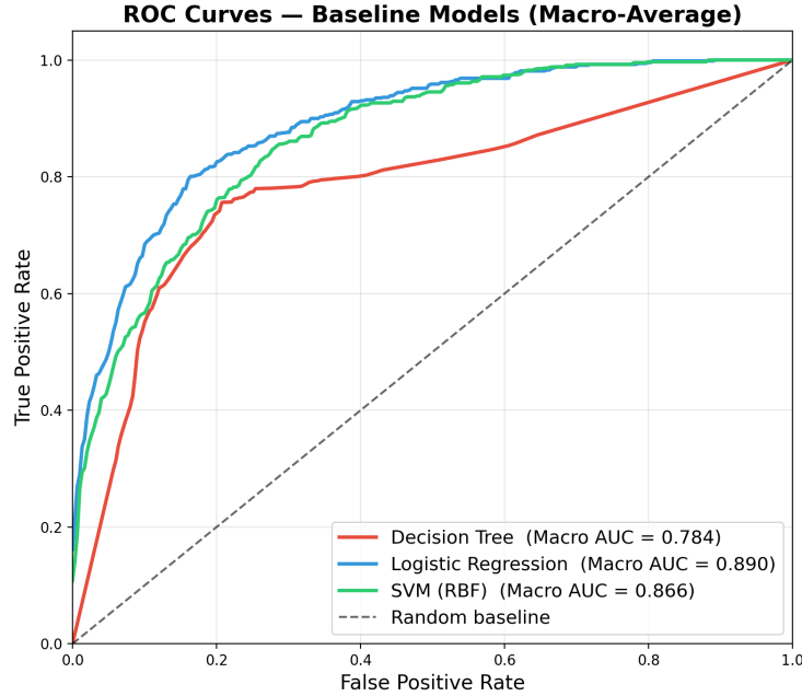
Figure 11: Macro-average ROC curves for all baseline models.
