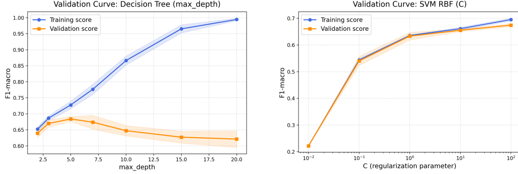
Figure 12: Validation curves: DT max_depth (left) shows overfitting; SVM C (right) shows improvement with larger C.
