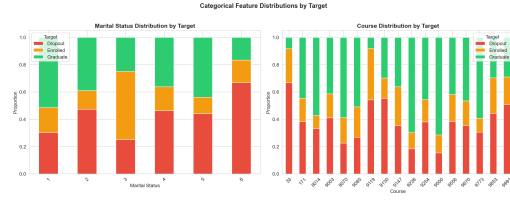
Figure 2: Categorical distributions stacked by target.
