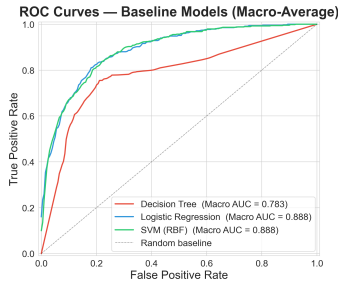
Figure 8: Macro-average ROC curves for all baseline models.
