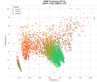
Figure 8: GMM (K=3)
