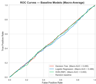
Figure 8: Macro-average ROC curves for all baseline models.
