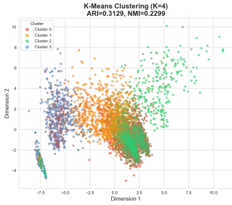
Figure 6: K-Means (K=4)
