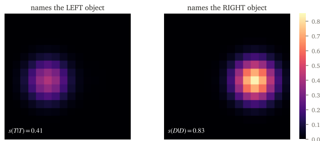
Figure 7: Two faces of one weight. Top: changing one word moves both the action target and the predicted region of motion to the newly named object (schematic). Bottom: the predicted motion mass over two objects, same pixels, one word changed; the mass moves two orders of magnitude (illustrative of the measured s(T|T)=0.41 , s(D|D)=0.83 ).
