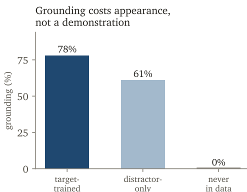
Figure 6: The scaling economics of the recipe: a new object needs only to appear in training scenes for its grounding to become learnable; no grasp demonstration of it is required. Target-trained 78%, distractor-only 61%, never-in-data 0%.
