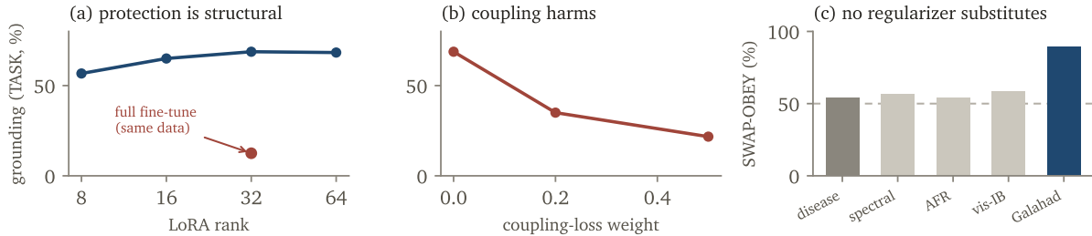
Figure 4: Only deconfounded data with low-rank protection installs grounding. (a) Protection is a property of the rank: the capacity curve rises then plateaus, and full fine-tuning on the same data collapses to 12.5%. (b) Coupling supervision harms in a dose-response. (c) Three training-time regularizers on confounded data all sit at the disease level; none approaches the deconfounded recipe.
