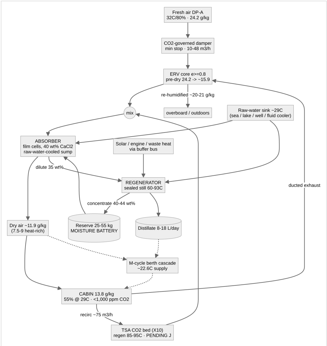
Detailed air-path diagram: diagrams/dpa-mixed-mode-airpath.svg .
