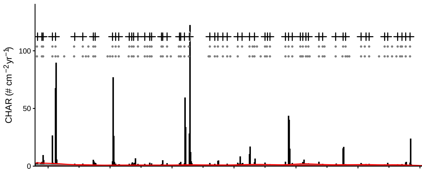
(b) Detection frequency and timing uncertainty (1000-chronology ensemble)
