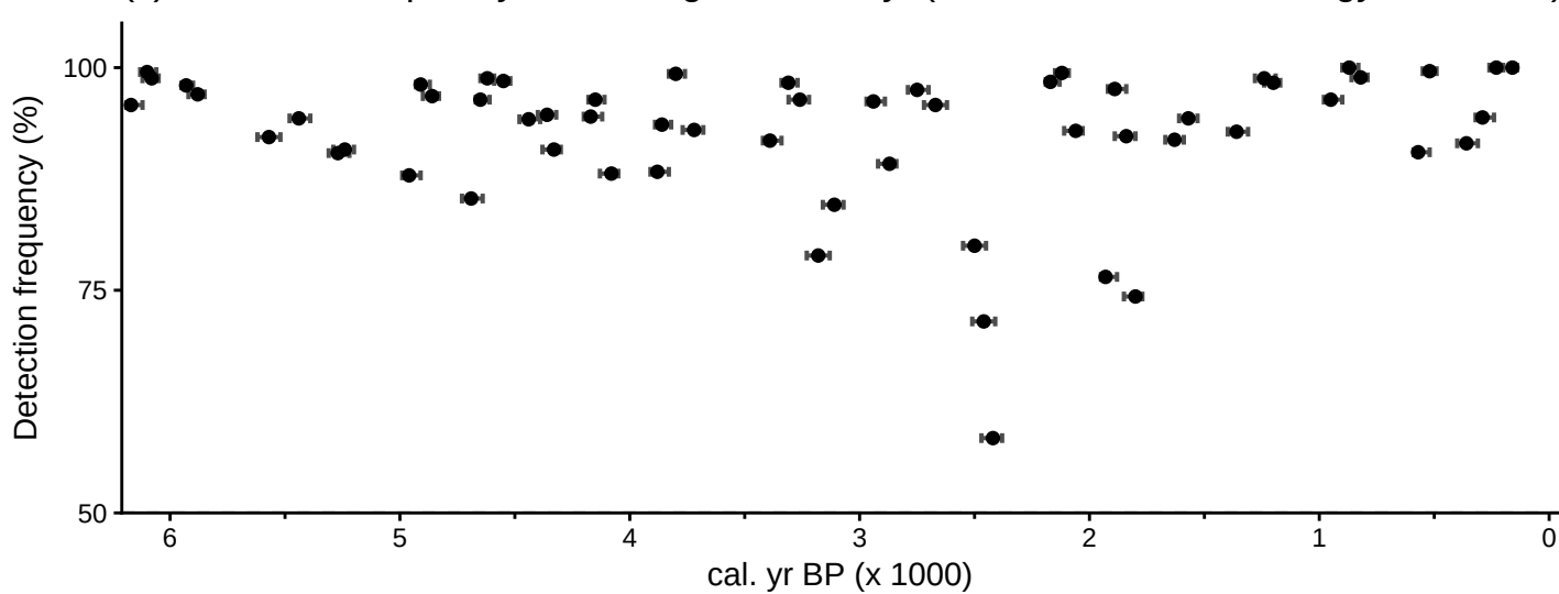
(c) Detection frequency and timing uncertainty (95% CI, 1000-chronology ensemble)
