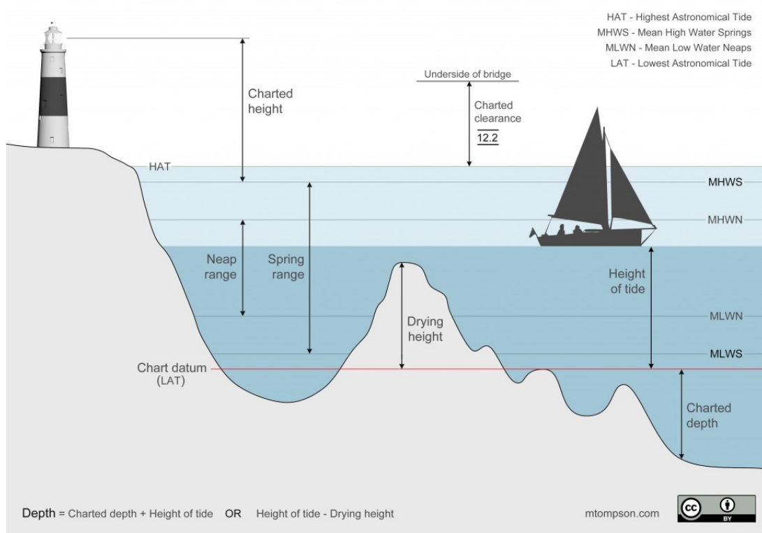
Figure 4.4: Tidal Heights
