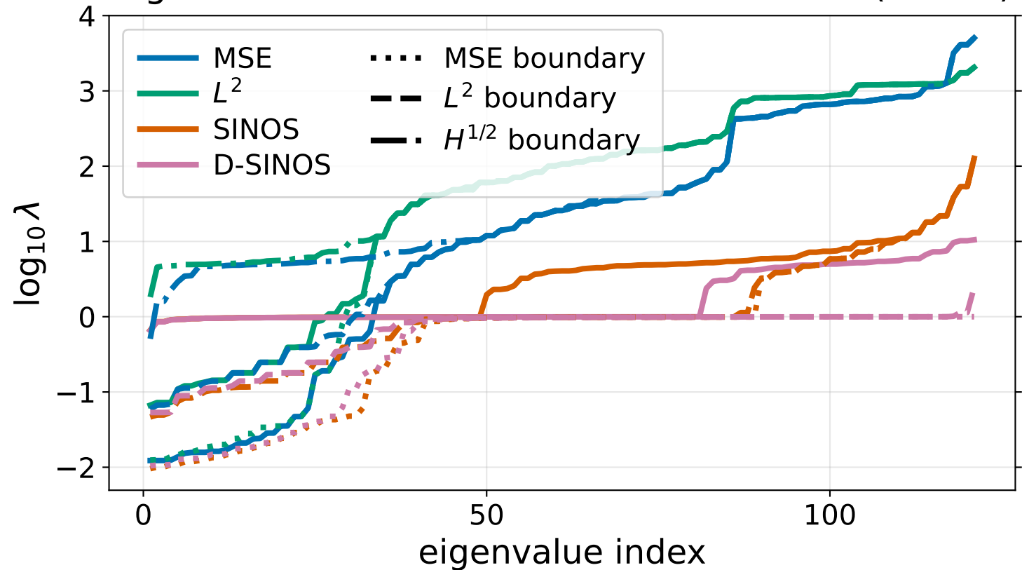
Eigenvalues of residual matrices w.r.t. H^1 ( n = 10 )
