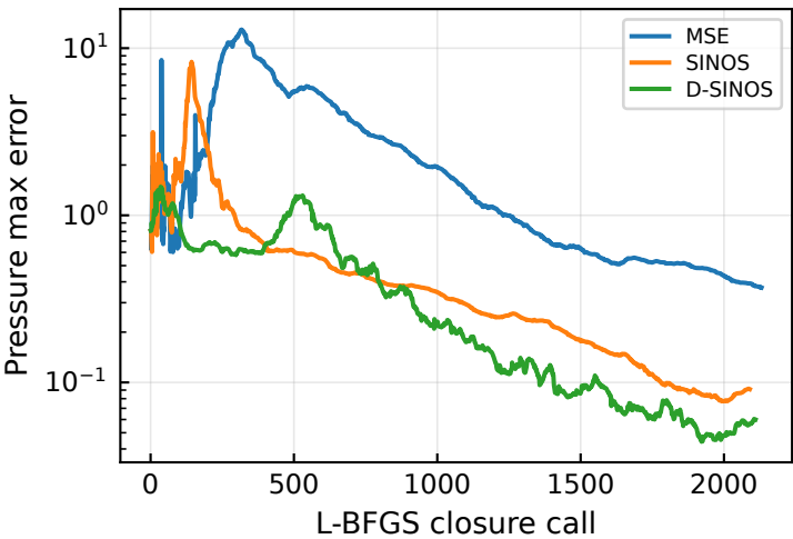
Pressure max error history
