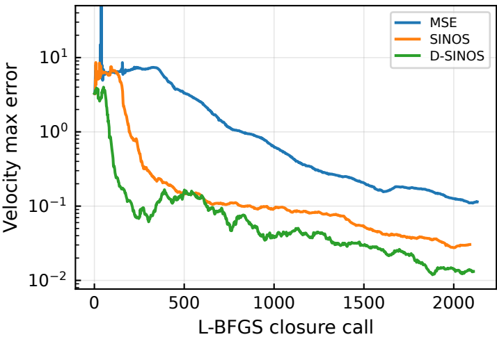
Velocity max error history
