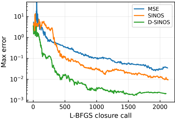
Max error history
