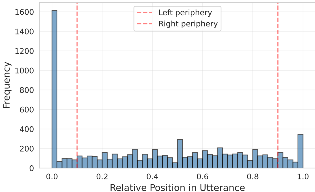
Discourse Marker Distribution (L/R = 2.72)
