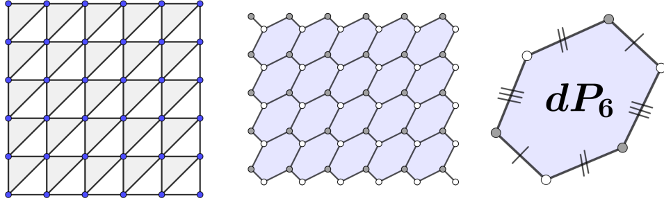
FIGURE 2. Left: \mathbb{Z}^2 -periodic tiling \mathcal{T} of the plane \mathbb{R}^2 . Middle: \mathbb{Z}^2 -periodic infinite quilt of smooth toric surfaces. Right: Its \mathbb{Z}^2 -quotient and the central fiber of Mumford construction, a glued dP_6 . Two 0-dimensional torus orbits in white and grey, three 1-dimensional torus orbits in black; the 2-dimensional torus orbit in blue.
