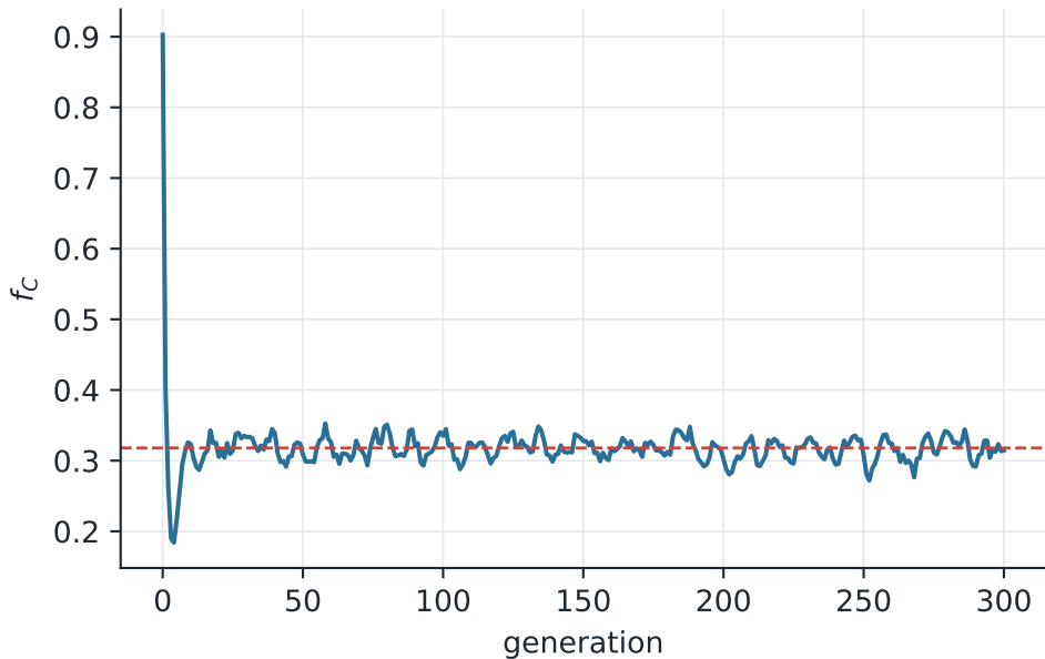
Cooperator fraction over time, b = 1.9 (dashed: 0.318)
