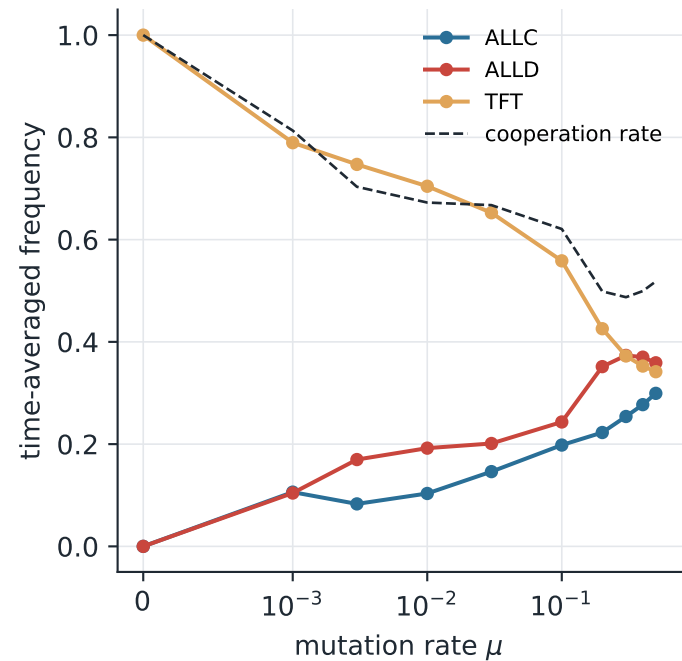
ALLC / ALLD / TFT, Moran N=50, start at TFT Mutation-driven cycles: ALLC drifts in, ALLD invades, TFT restores
