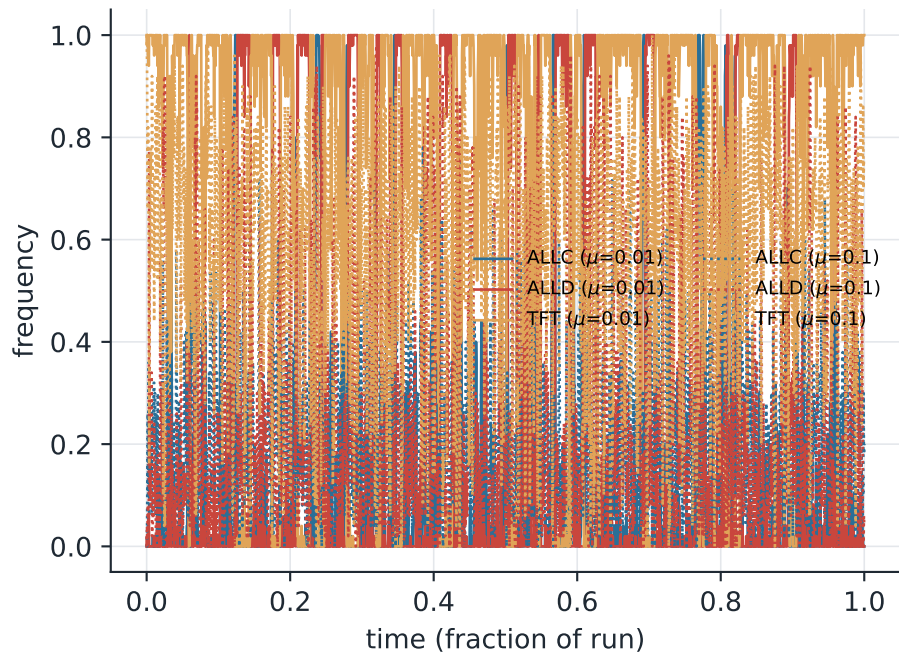
ALLC / ALLD / TFT, Moran N=50, start at TFT Mutation-driven cycles: ALLC drifts in, ALLD invades, TFT restores
