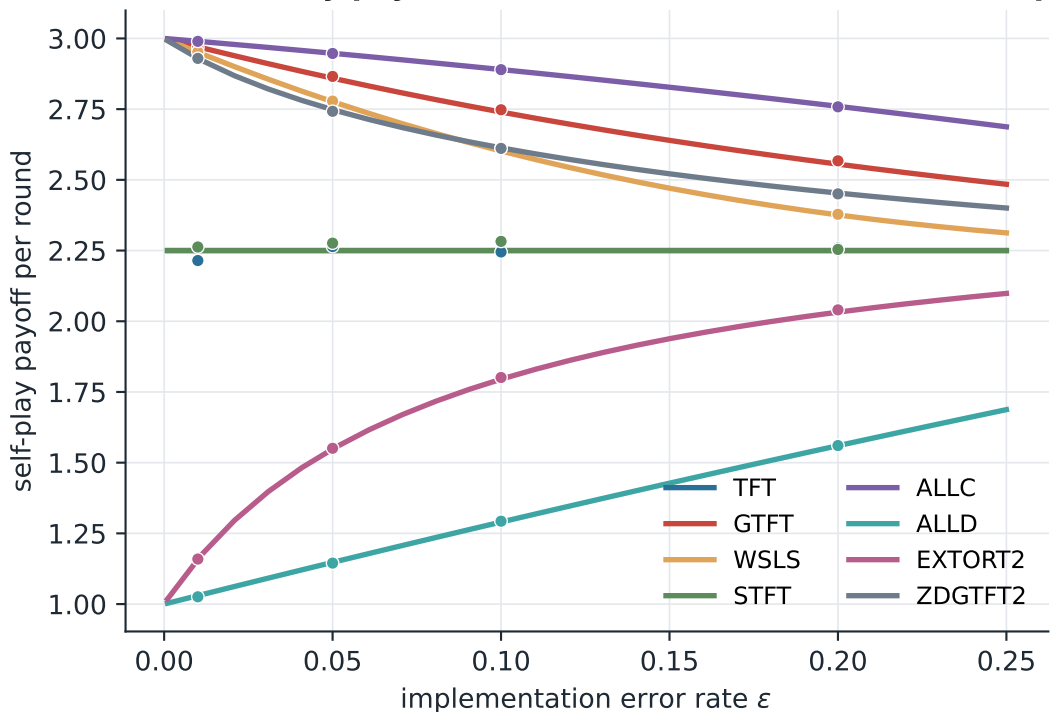
Exact stationary payoff (lines) vs simulation (dots) in self-play
