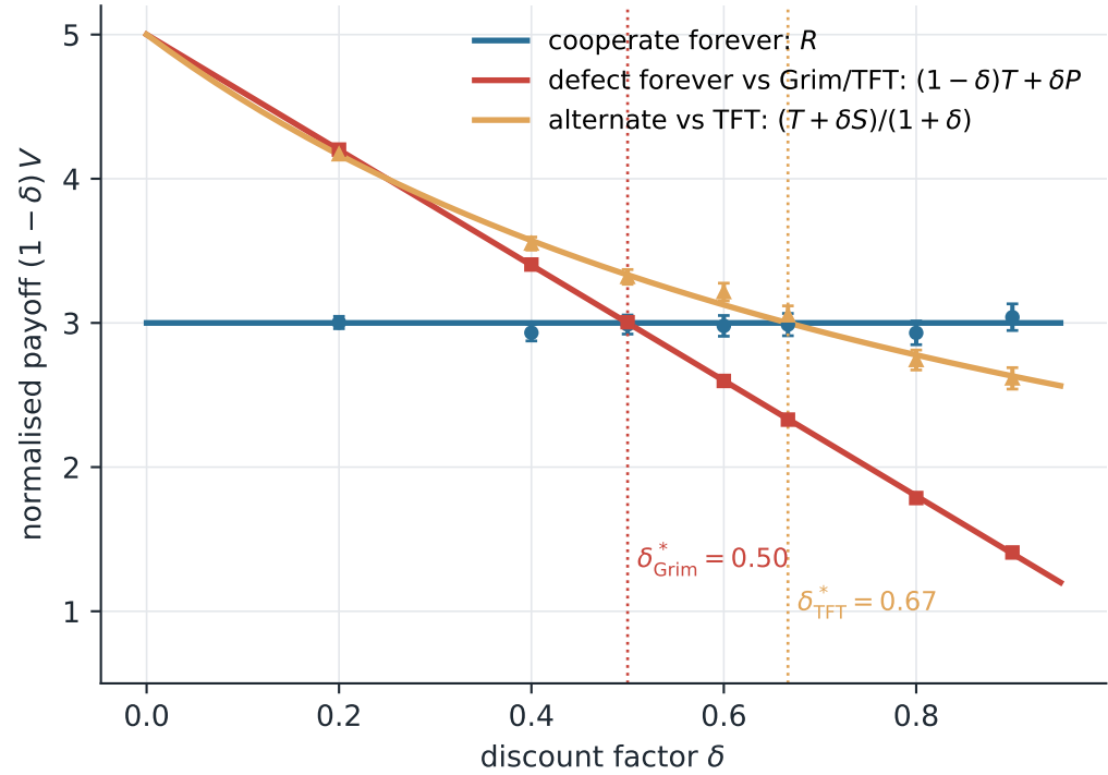
Cooperation vs. deviation (lines: exact; markers: geometric-stopping simulation, \pm 2 s.e.)
