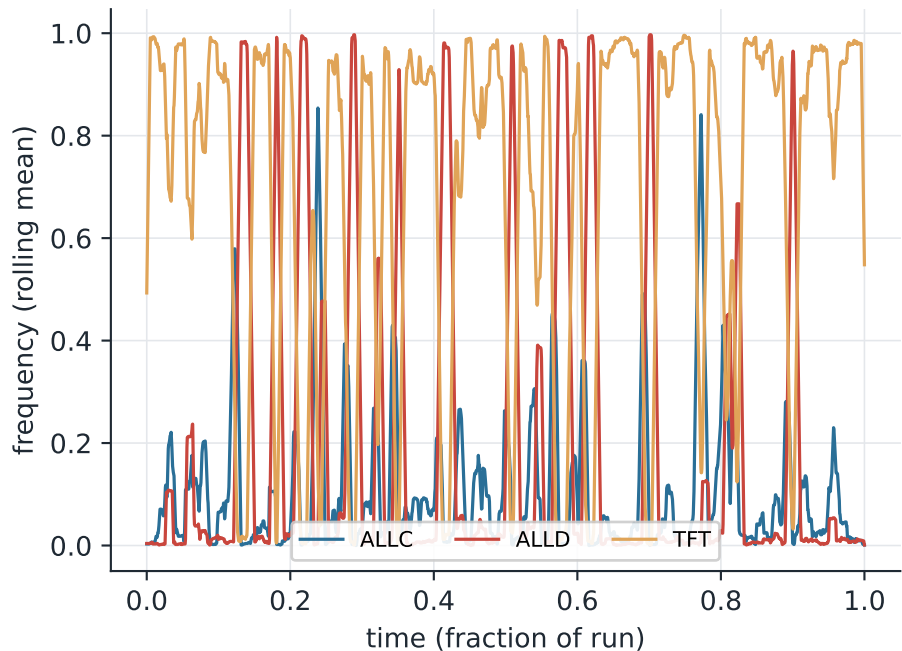
\mu = 0.01 : ALLC drifts in, ALLD invades, TFT restores
