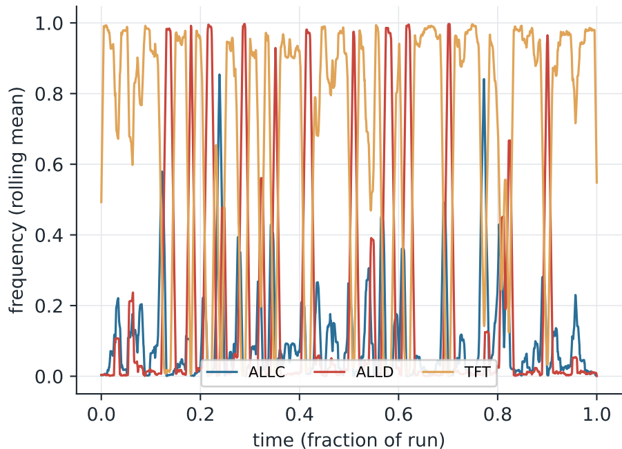
\mu = 0.01 : ALLC drifts in, ALLD invades, TFT restores
