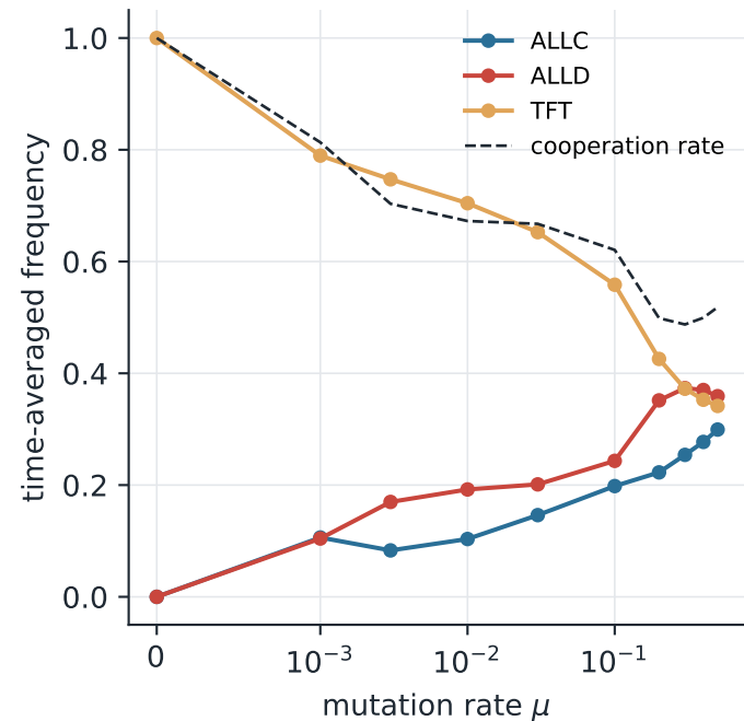
Moran N=50, from all-TFT
