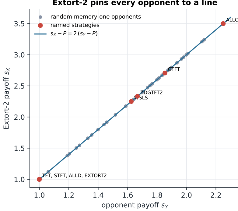
Figure 14: Without noise, Extort-2 confines every opponent to the line s_X - 1 = 2(s_Y - 1) (grey: random memory-one opponents; red: the named strategies).
