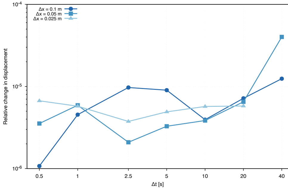
Steady-state displacement convergence
