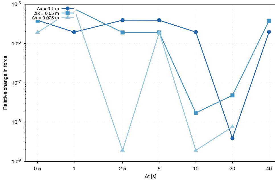
Steady-state force convergence
