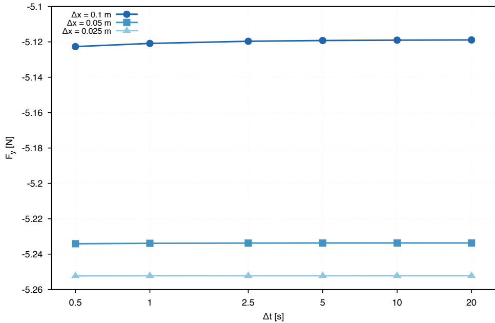
Force sensitivity to time step
