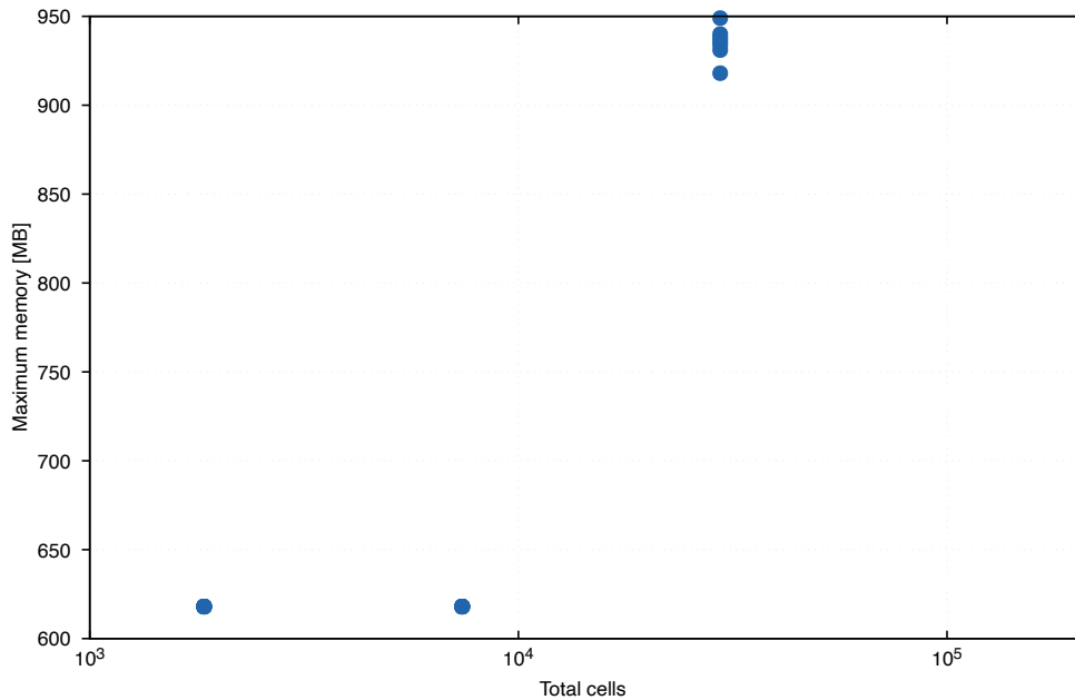
Memory usage versus problem size (monolithic, default)
