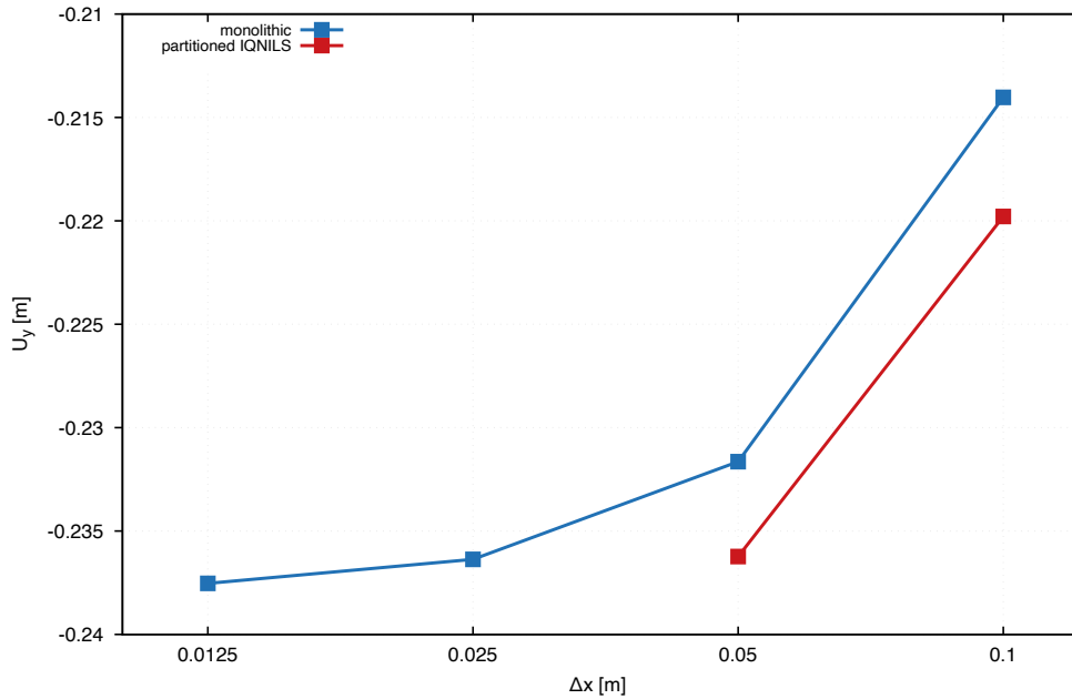
Displacement sensitivity to mesh size (all schemes, \Delta t = 1 s)
