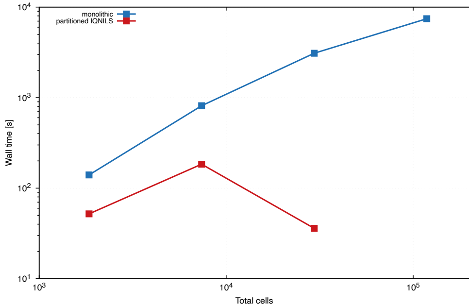
Wall time versus problem size (all schemes, \Delta t = 1 s)
