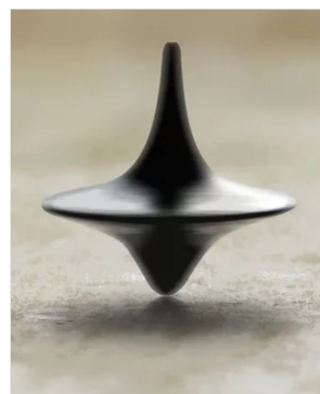
20 Inception
