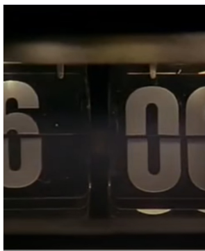
6 Groundhog Day
