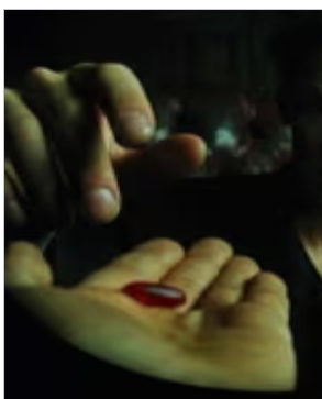
17 The Matrix
