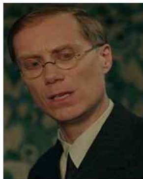
24 Stephen Merchant
