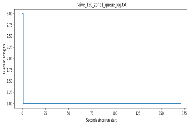
Figure 8. Server queue length over time, zone 1 (naive, T=50ms ).
