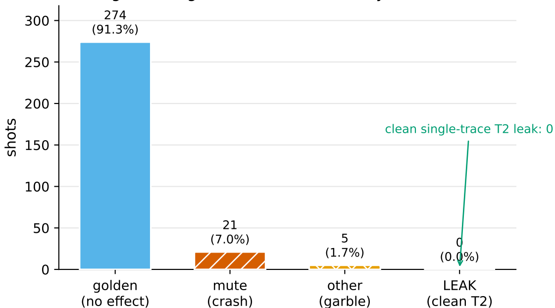
Single clock-glitch on real HAETAE +y (T2), N=300
