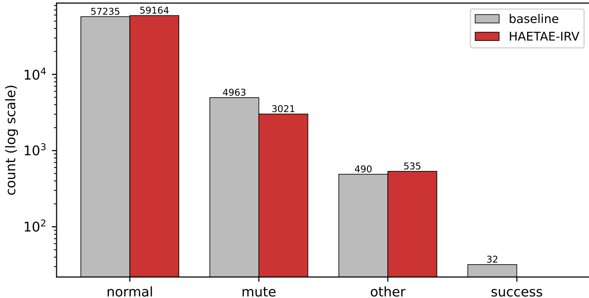
Outcome distribution: baseline vs HAETAE-IRV (N=62,720 each)
