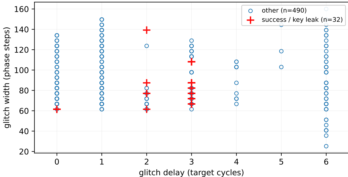
Baseline: clock-glitch parameter map (T2 key-leak region)
