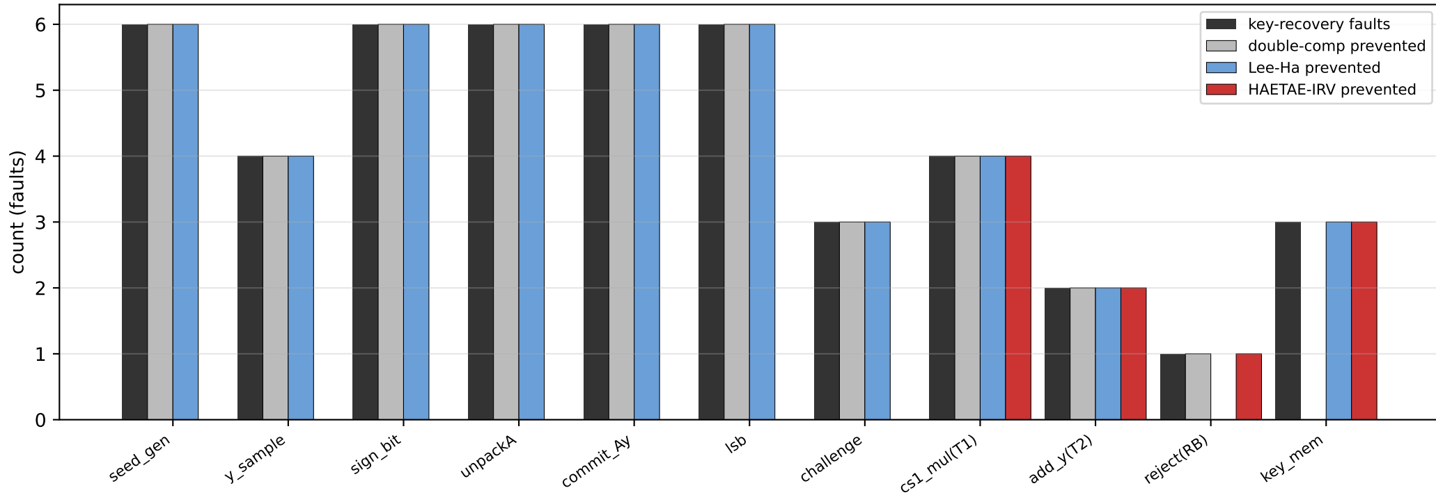
Per-line key-recovery faults and prevention (real full HAETAE sign, x86)
